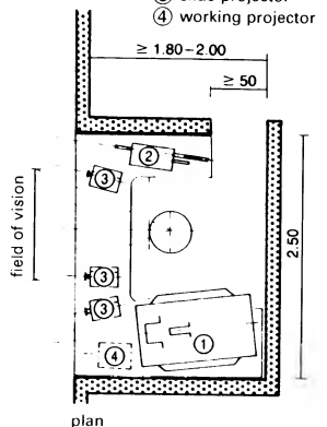
⑦ Projector room
